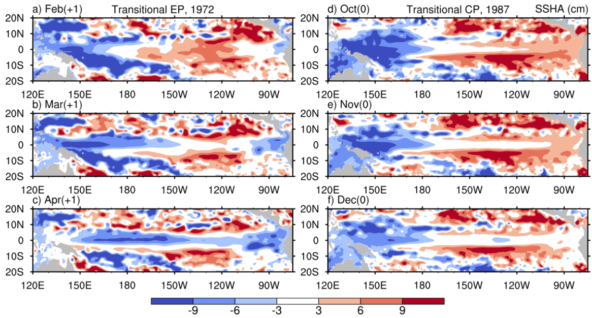
Figure S8. Temporal evolutions of SSHA anomalies for (a, b, c) the transitional EP El Niño event in 1972/73 and (d, e, f) the transitional CP event in 1987/88.
