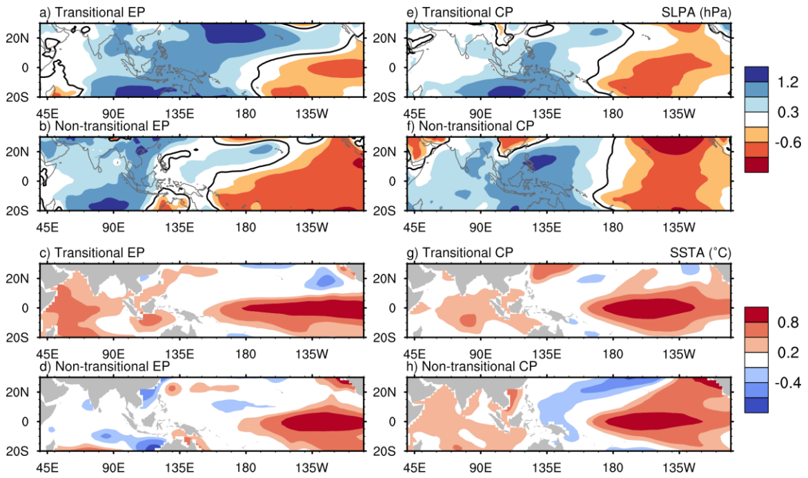
Figure S10. As in Figs. 3a, 3b, 3d, 3e, 3g, 3h, 3j and 3k, except for the anomalies from the JRA-55 and NOAA ERSST V5.
